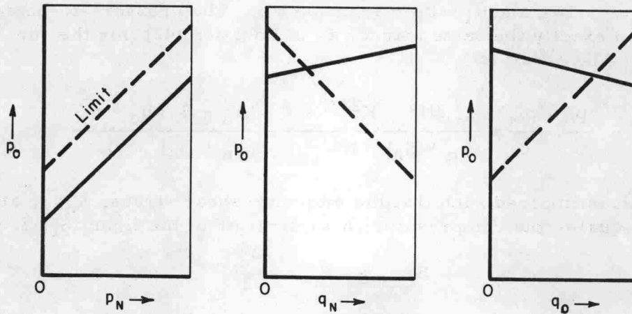
FIGURE 63. INFLUENCE OF PRESSURES p_N , q_N AND q_o ON THE PRESSURE CAPABILITY p_o
